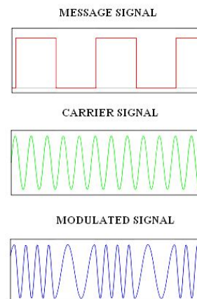
Figure 1: Frequency Shift Keying Modulation
