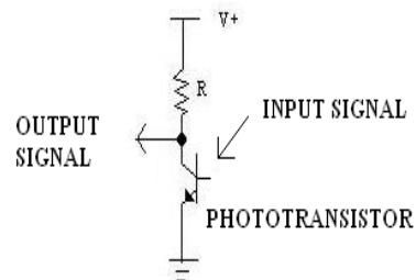
Figure 10: Receiver using Phototransistor
