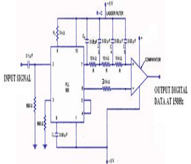
Figure 12: Demodulator using PLL 565
