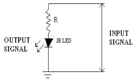
Figure 8: Transmitter using IR LED
