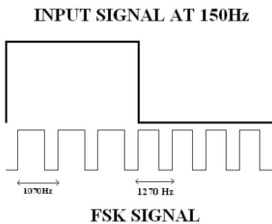
Figure 6: FSK modulated signal
